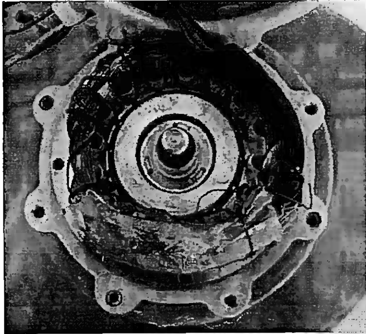
<Motor winding view>
